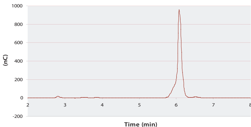
Chromatogram of ProG JBG-002 at 108 ppm
